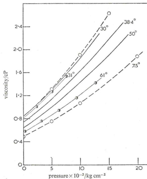
FIG. 8.—The viscosity of carbon tetrachloride. \circ , Van Wijk et al. ; \circ , Bridgman 7 ; —, this work.
